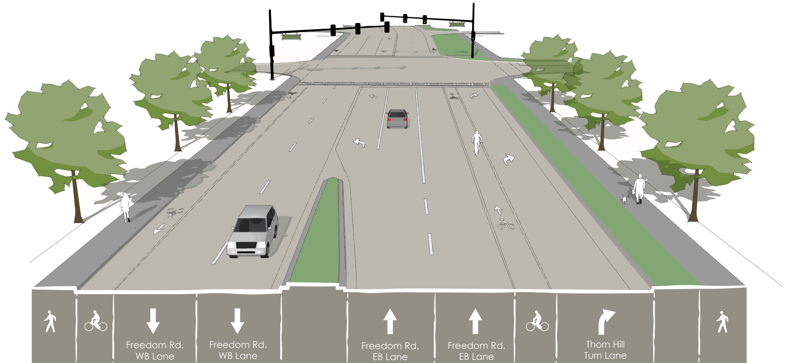
Proposed Freedom Rd. & Thorn Hill Rd. Intersection
